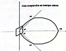
Fig. 5. Radiation pattern schematic for a patch antenna [9]
