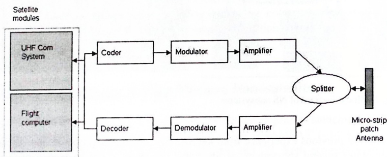
Fig. 3 Block diagram of NS subsystems
